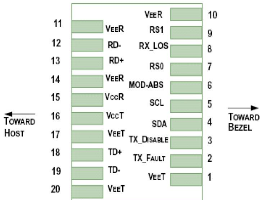
Figure1.Elecctrical Pin-out Details
