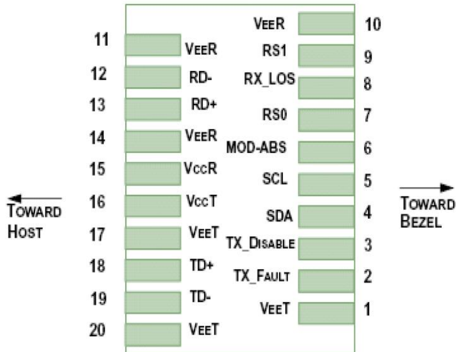
Figure1.Elecctrical Pin-out Details
