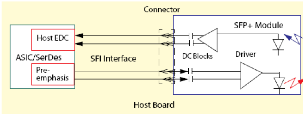
Figure 1: Interface to Host
